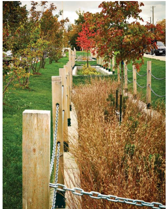
Elm Drive in Mississauga has been retrofitted according to LID practices. Rainwater is directed through permeable pavers into bioretention cells (rain gardens). In these cells, water is cooled and filtered before it infiltrates into the ground.
